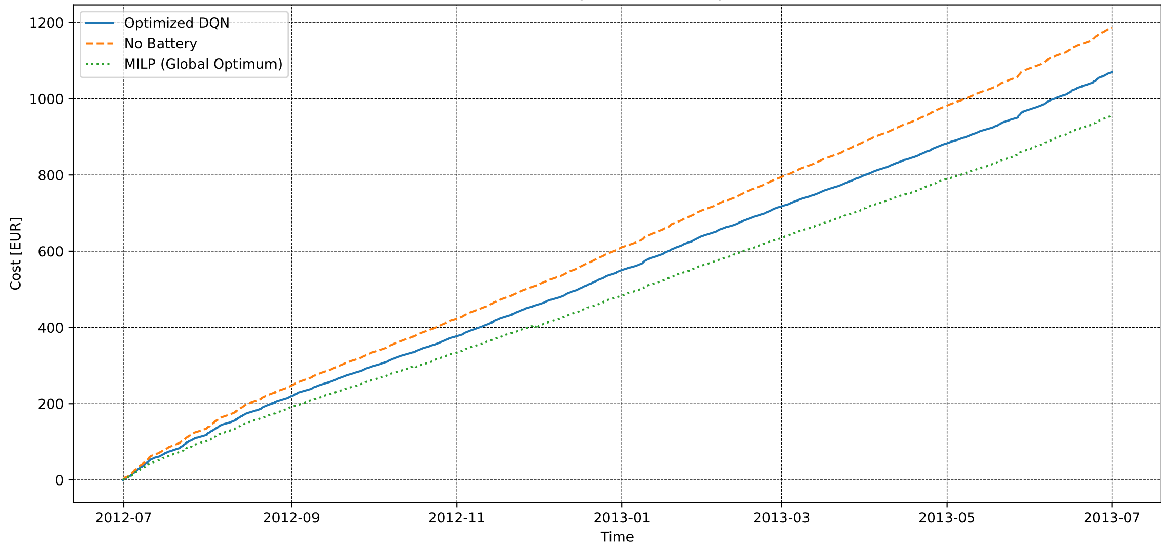
User 261 - Extended Convergence - Electricity Cost [DQN vs MILP]
